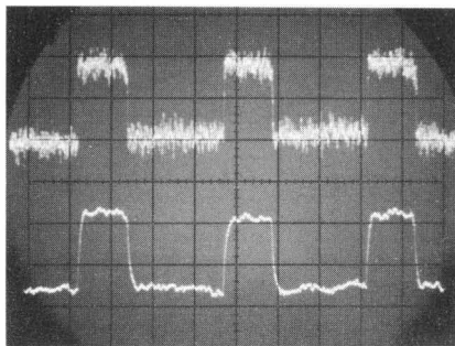
Fig. 2. Adjustable bandwidth of high-sensitivity plug-ins can be used to improve signal-to-noise ratio of low frequency signals, as in this double-exposure oscillogram.
