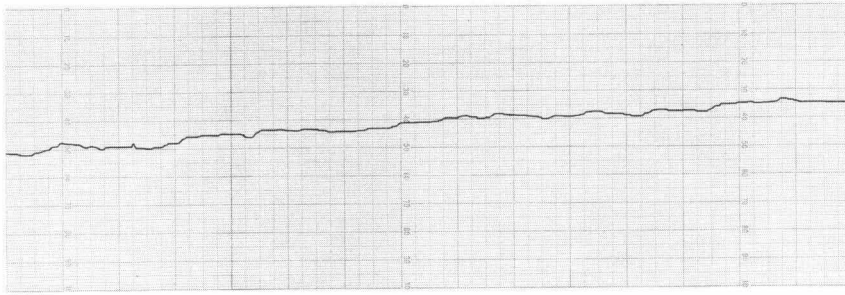
Fig. 4. High stability of Model 1400A 100 \mu\text{v}/\text{cm} amplifier is shown by one-hour recording of dc drift. Major vertical divisions represent 0.1 \text{ mv} referred to plug-in input, indicating drift of less than 0.2 \text{ mv}/\text{hour} after warm-up.
