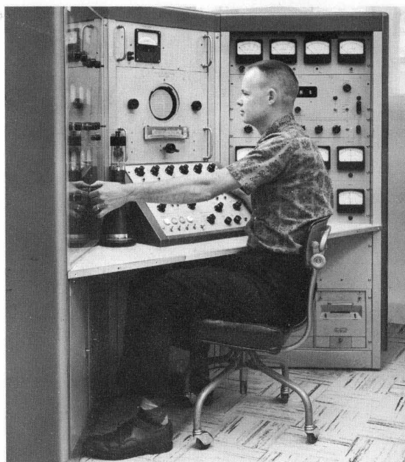
Cathode-ray tube in new oscilloscope is produced in -hp- CRT facility. Tube designer David Chaffee checks tube performance at test console.
