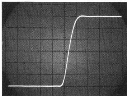
Fig. 2. Oscillogram of step response of Model 1402A dual-channel 20-megacycle plug-in operating in Model 140A Oscilloscope. Sweep speed is 20 nsec/cm.
