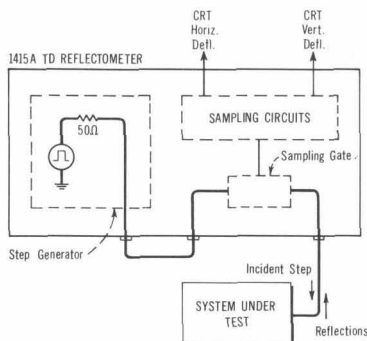
Fig. 5. Step generator in Reflectometer has 50 ohm source impedance which absorbs reflections traveling back through Sampling Gate.
