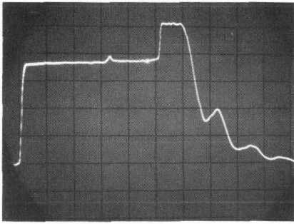
Fig. 4. Antenna system is examined here with Time Domain Reflectometer. Various impedance discontinuities can be identified separately and located by position on trace. Shape of reflection discloses nature of discontinuity.
