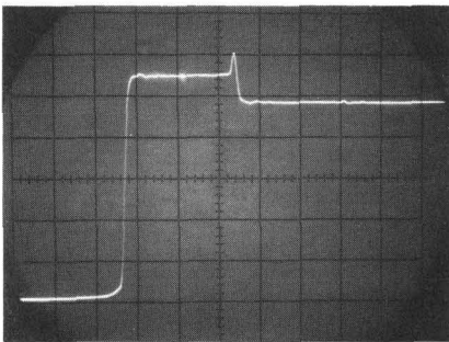
Fig. 2. Impedance mismatch between 50-ohm coaxial cable and 39-ohm termination is shown by this oscillogram made with -hp- Model 140A oscilloscope and Model 1415A Time Domain Reflectometer plug-in. Sharp spike results from inductance of termination leads. Bright dot corresponds to setting of calibrated dial on delay control, permitting quick location of discontinuities. (Sweep speed: 4 nsec/cm)
