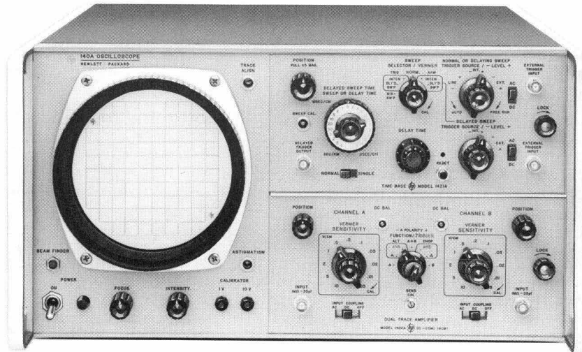
Fig. 1. For maximum flexibility, new -hp- Model 140A Oscilloscope has all deflection circuitry in plug-ins. Measurement range spans dc to 20 Mc and sensitivities to 10 \mu\text{v}/\text{cm} .
