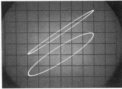
Fig. 6. Dual X-Y displays can be obtained with new oscilloscope, as shown by above single-exposure oscillogram comparing phases at two different places in test circuit.
